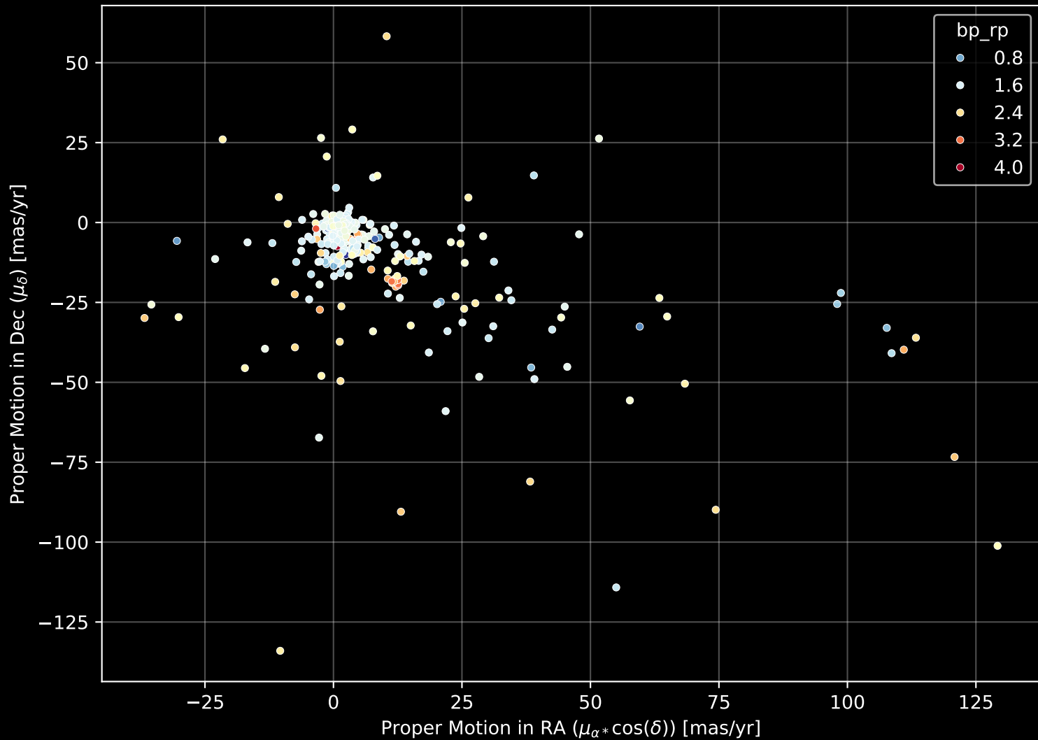
APOGEE DR17 Field: [TAUL1551_btx] Proper Motion Diagram (n= 374)
