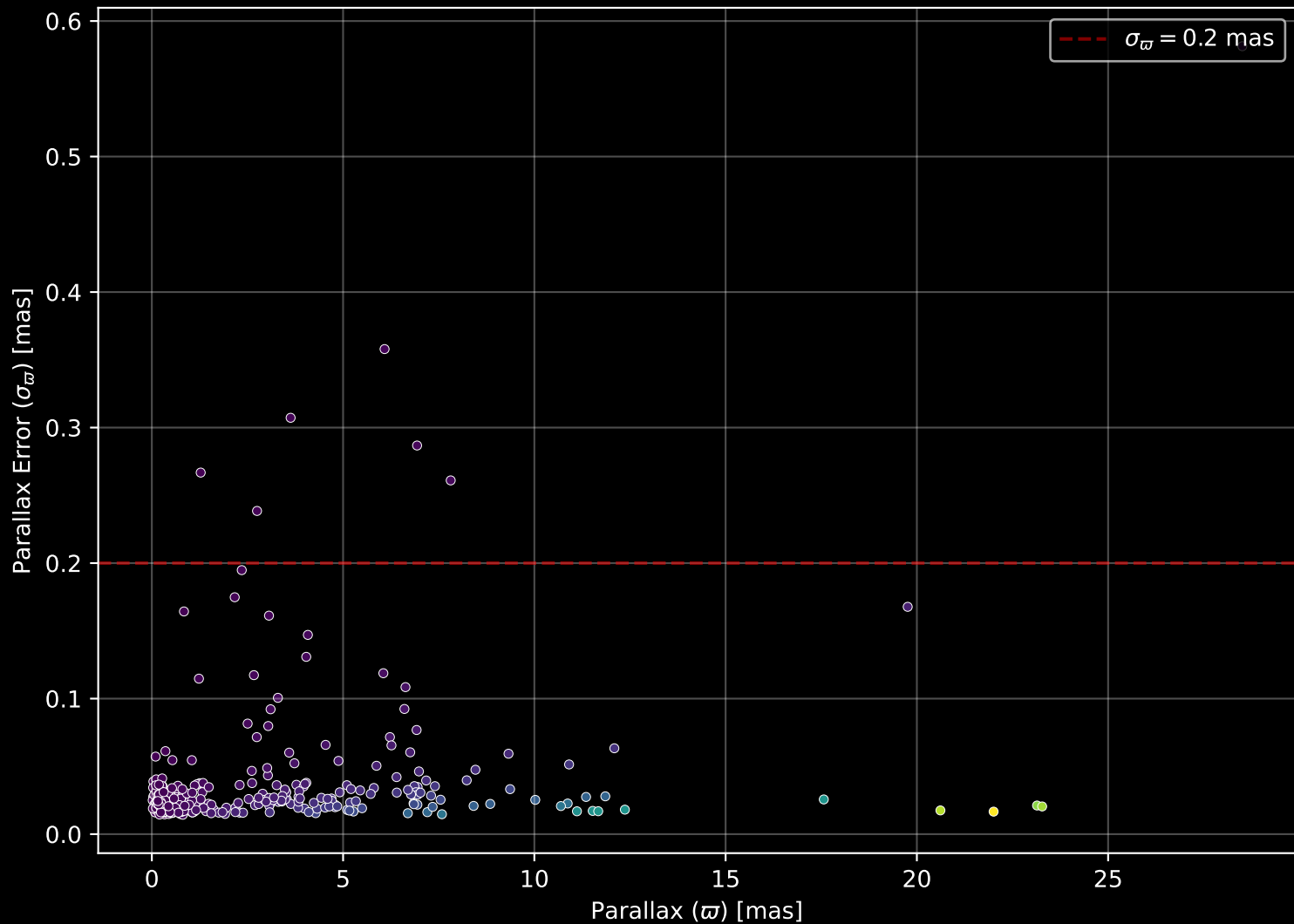
APOGEE DR17 Field: [TAUL1551_btx] Parallax Quality (n= 374)
