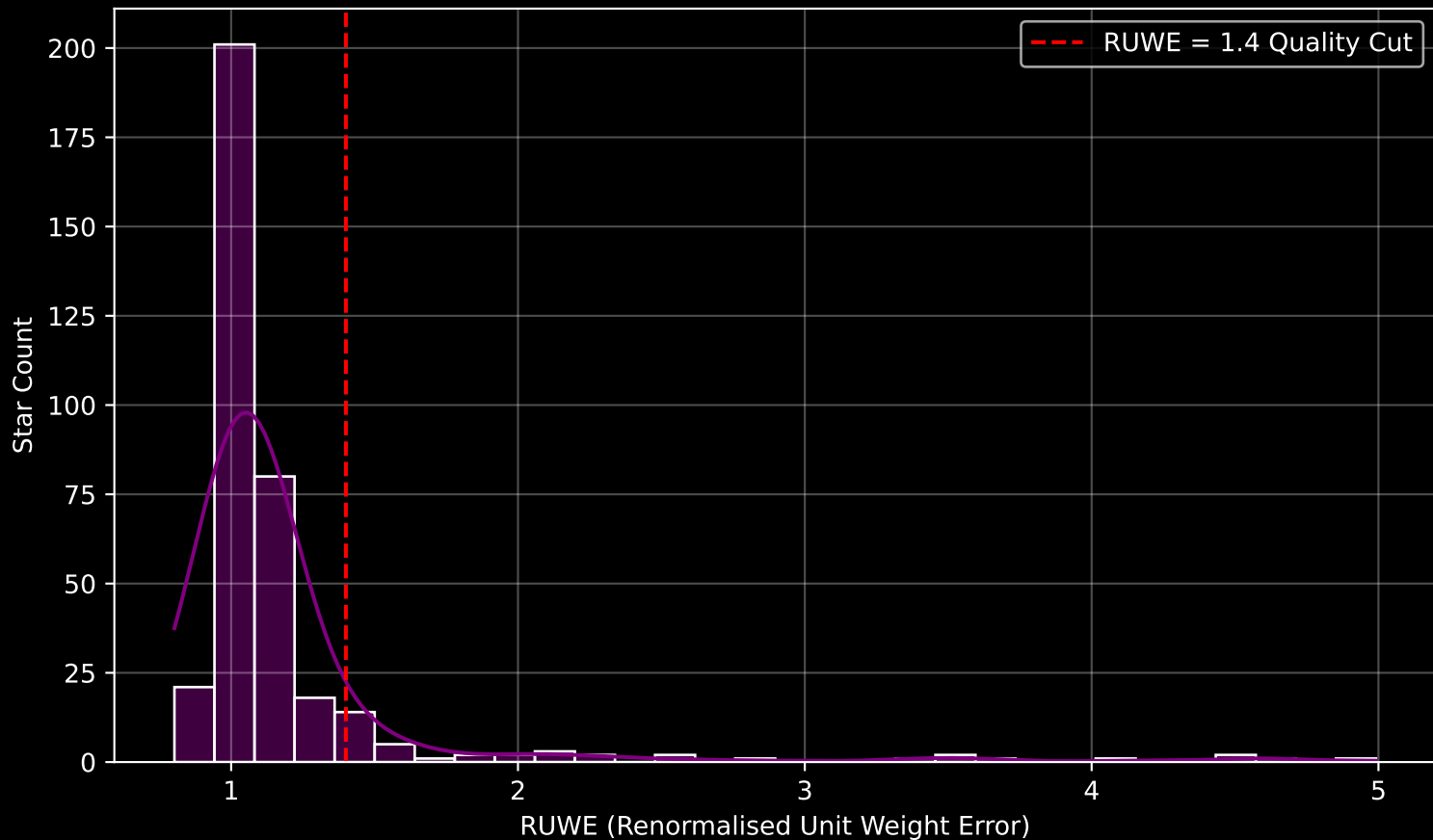
GAPOGEE DR17 Field [TAUL1551_btx] RUWE Distribution (n= 361)
