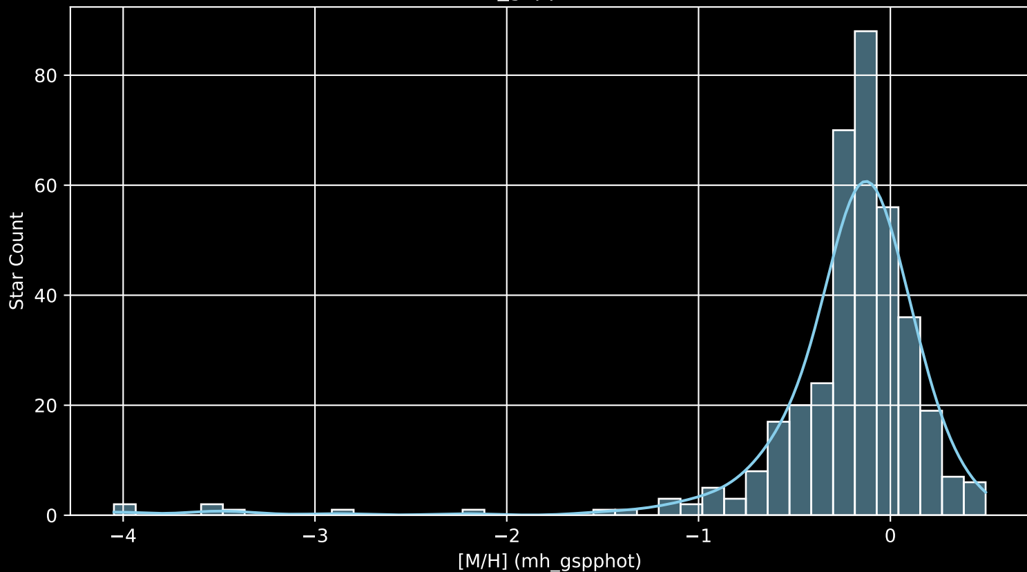
APOGEE DR17 Field: [TAUL1551_btx [M/H] (mh_gspphot) (n= 373)
