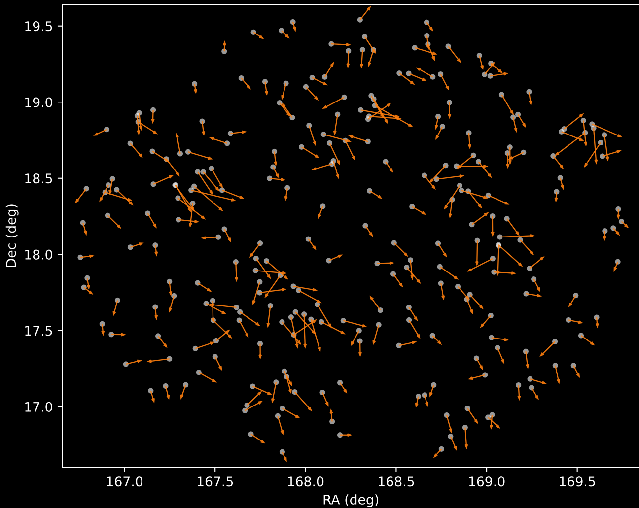
APOGEE DR17 Cluster 2 Proper Motion Vectors (n=255)
